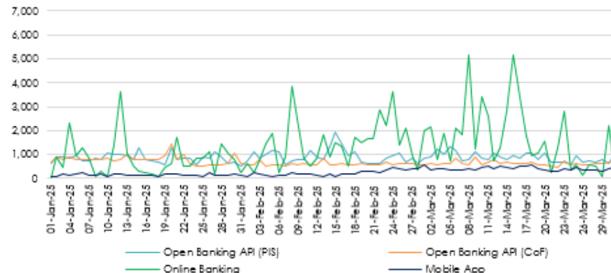
Payment Initiation performance (average response in milliseconds)
